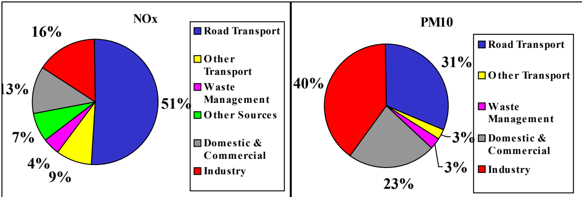
Figure 14. Proportion of emissions of NO x and PM 10 in the City of Paris
