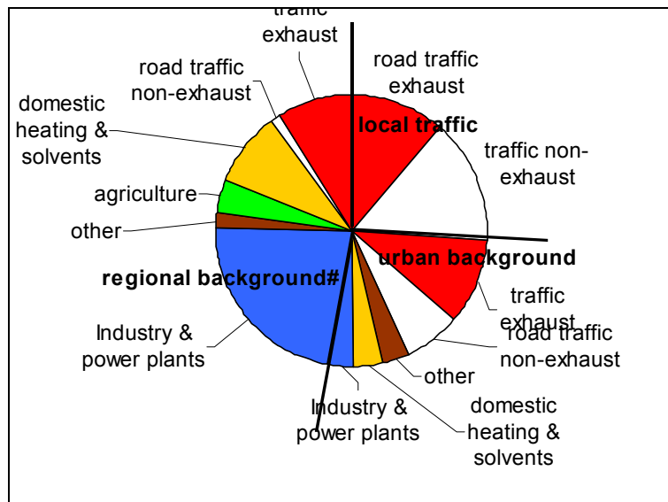
Figure 12. Estimated contribution to PM 10 at a busy traffic spot from all sources for Berlin in 2002 (also accounting for secondary sources of PM)
