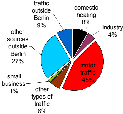
Figure 13. Modelled contribution to NO 2 urban background concentrations from all sources for Berlin in 2002
