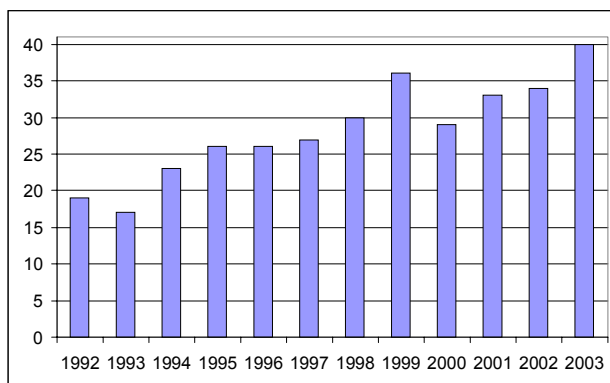
Figure 9. Recent annual average ozone measurements in Paris
