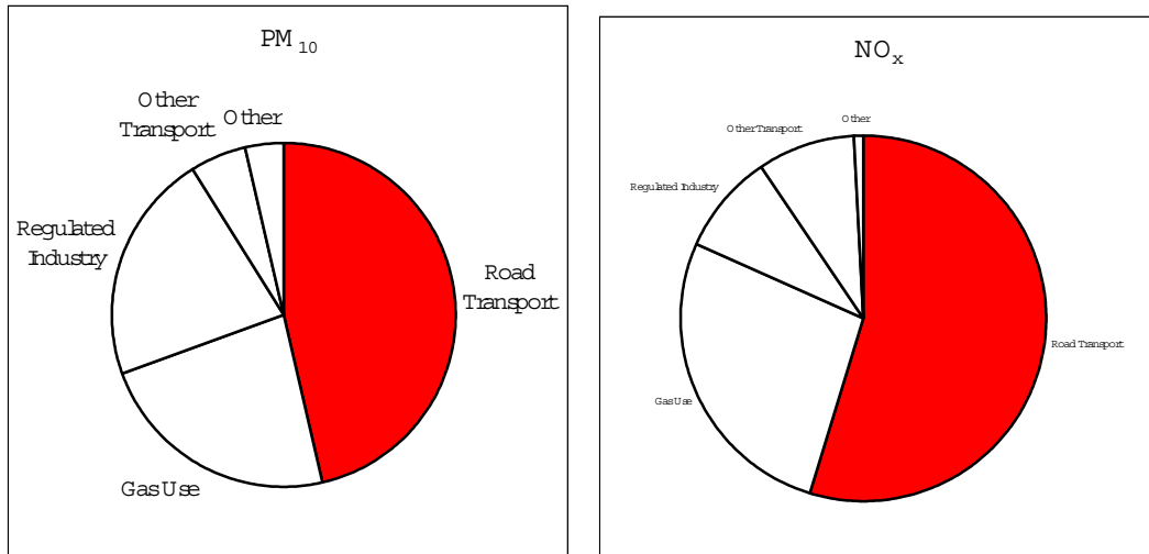
Figure 11. Proportion of emissions of NO x and PM 10 from different sources within Greater London in 2001
