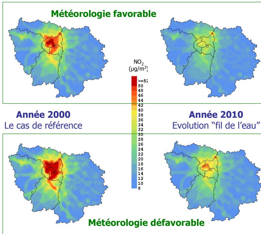
Figure 8. Modelling of NO 2 in Paris for 2000 and business as usual in 2010, with both favorable and unfavorable weather 19
