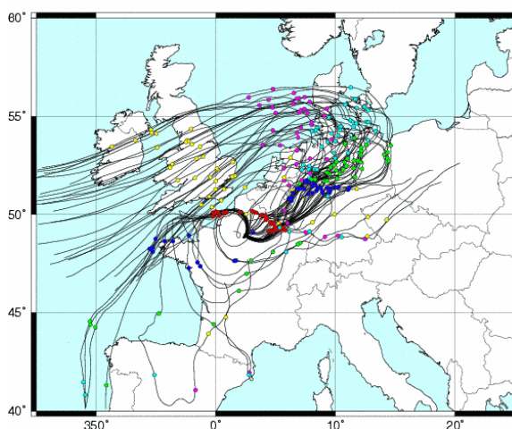
Figure 10. Backward-trajectories for an ozone episode in Paris on the 7 th August 2003
