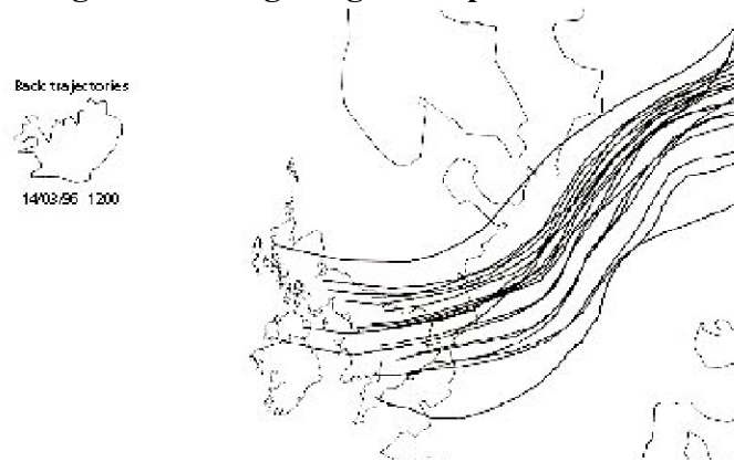
Figure 15. Long-range transport of PM 10 23
