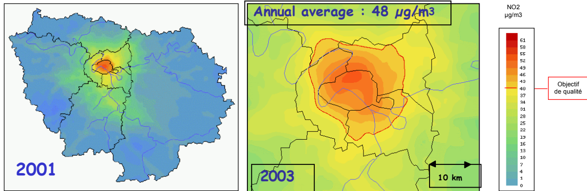
Figure 6. Modelled NO 2 concentrations in 2001 for the whole of Paris and 2003 for central Paris
