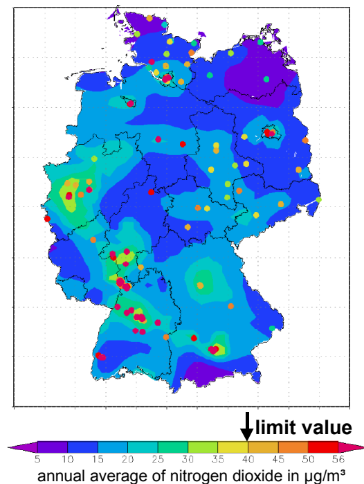
Figure 1. Measured distribution of annual NO 2 concentrations in Germany in 2002. The coloured areas are based on interpolated data of rural and background measurements, while the spots depict values recorded by traffic sites. 7
