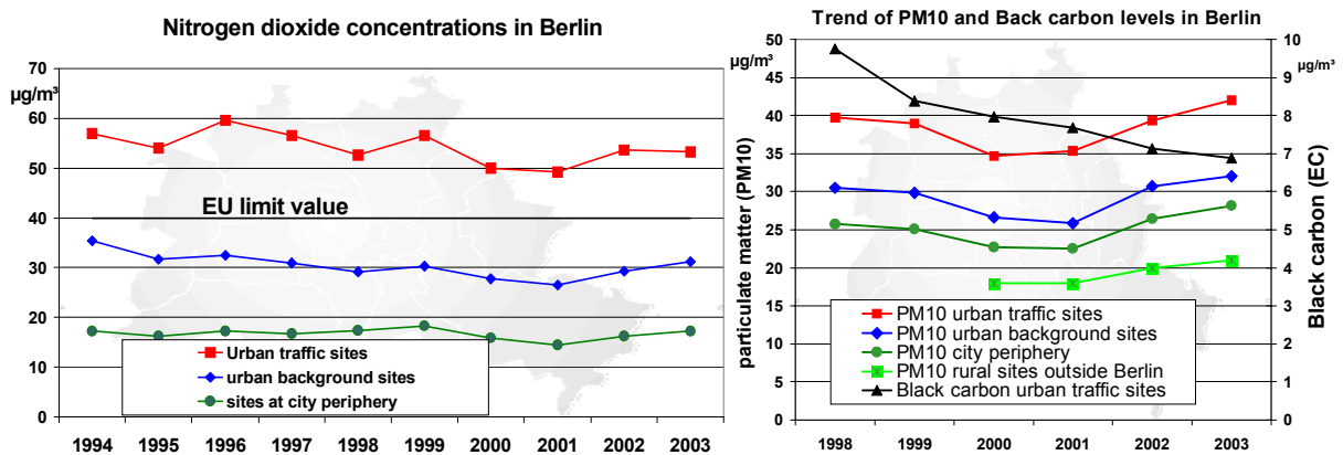
Figure 5. Recent trend of the annual average PM 10 and NO 2 concentrations at the periphery, urban background and traffic hot spot locations in Berlin
