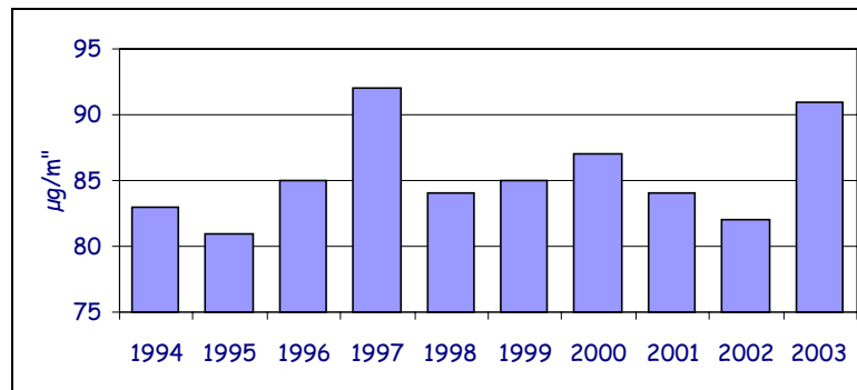
Figure 7. Recent measured NO 2 roadside average in Paris 18 (Note: the scale on the left starts at 75µg/m 3 )
