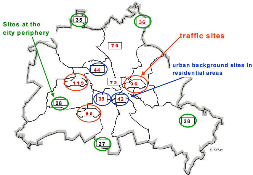
Figure 8. Monitored PM 10 levels in Berlin in 2003
